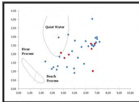
Figure 6 - Diagram of Stewart (1958).
