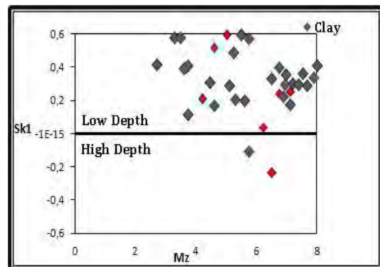
Figure 7 - Diagrams of Valia & Cameron (1979).
