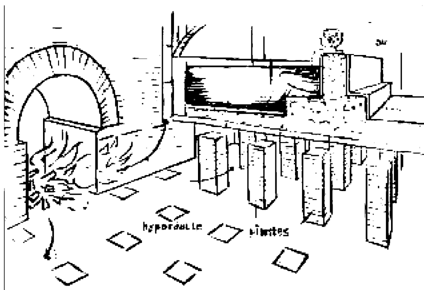
Σχ. 8. Suspensura κατὰ F. Yegül
