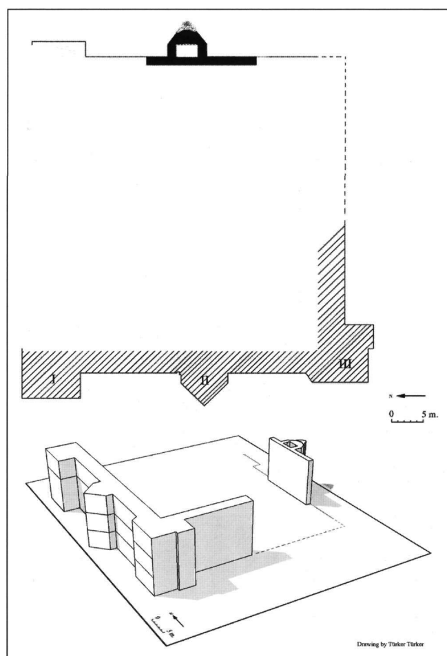
Fig. 5. Plan of Gallipoli Castle (Drawing by Turker Turker).
