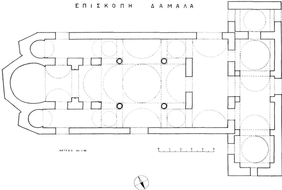
Εἰκ. 8. Κάτοψις τοῦ ναοῦ μετὰ τὴν ἐπέκτασιν τοῦ Ἱεροῦ καὶ τὴν προσθήκην ἐξωνάρθηκος.
