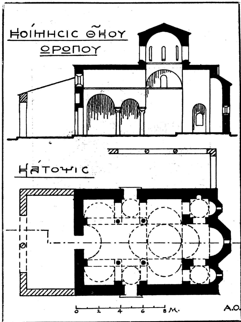
Εἰκ. 10. Κάτοψις καὶ τομὴ ναοῦ Κοιμήσεως Θεοτόκου ἐν Ὁρωπῶ.
