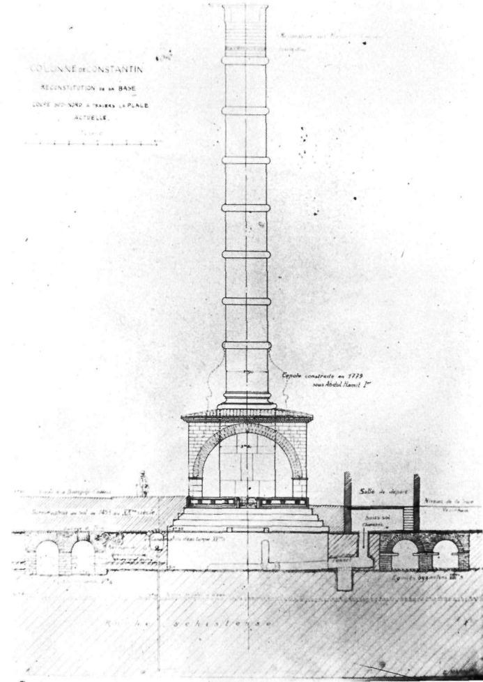
a. Plan of Constantinian's Column and Surrounding Area. b. Reconstructed Elevation of Constantinian's Column by E. Mamboury. German Archaeological Institute, Istanbul.
