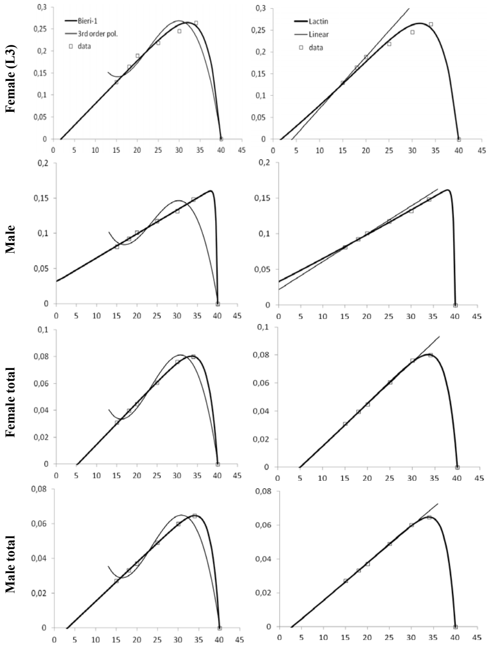
FIG 1 (continued from the foregoing page). Relationship between development rate ( d^{-1} ) of different stages and temperature ( ^{\circ}C ) for P. solenopsis .
