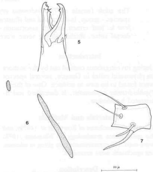
FIGS. 5-7. Typhlodromus erymanthii spec. nov., female: 5 chelicerae, 6 primary and secondary metapodal plates, 7 basitarsus IV.
