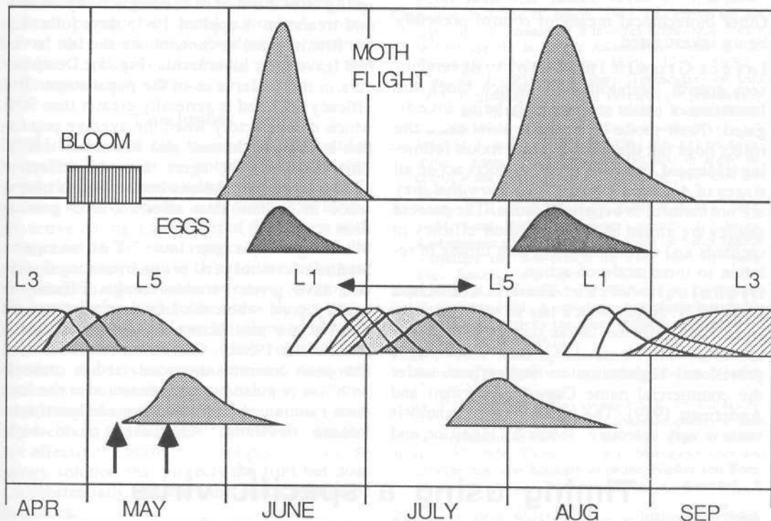
FIG. 4. The optimum timing of IGR products, for example fenoxycarb, in relation to the occurrence of sensitive life stages of Adoxophyes orana F.v.R. under conditions in Switzerland.
