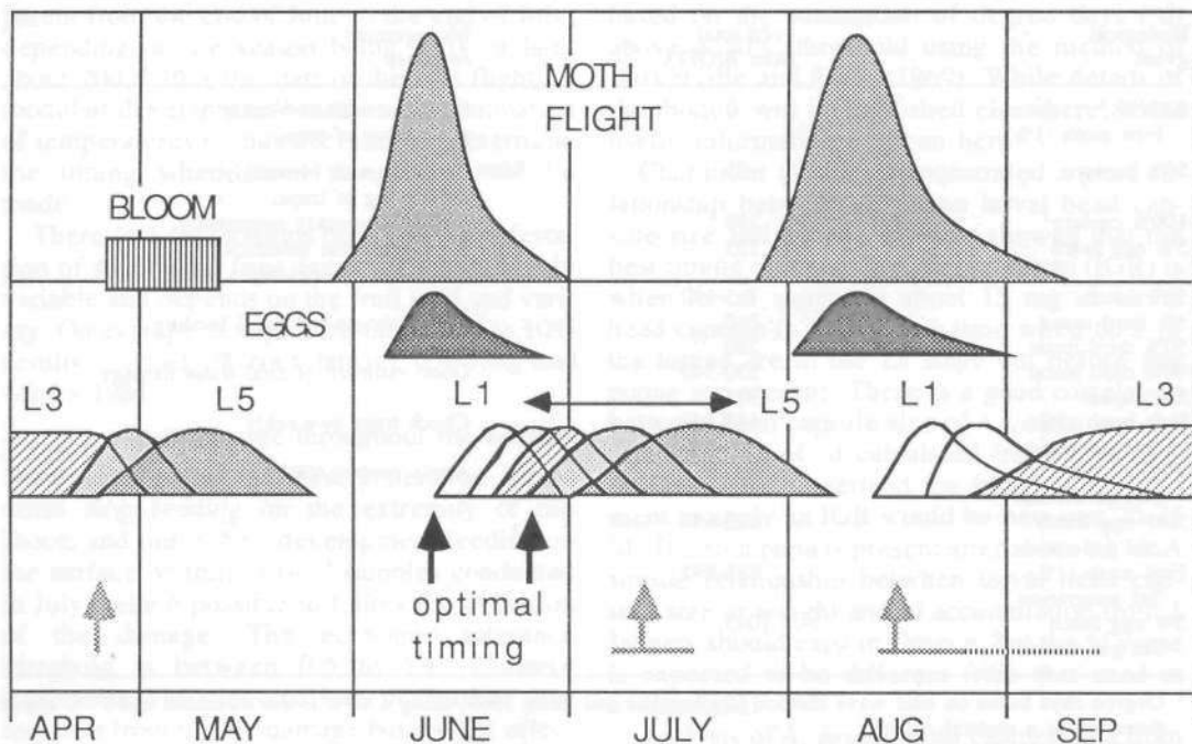
FIG. 3. Timing of classical insecticides in relation to the occurrence of sensitive life stages of Adoxophyes orana in Switzerland. The optimal timing is represented by the black arrows while alternative timings are shown as shaded arrows.
