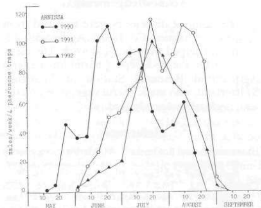
FIG. 2. Weekly captures of Synanthedon myopaeformis males in four pheromone traps in the untreated apple orchard (C). Armissa in 1990-1992.
