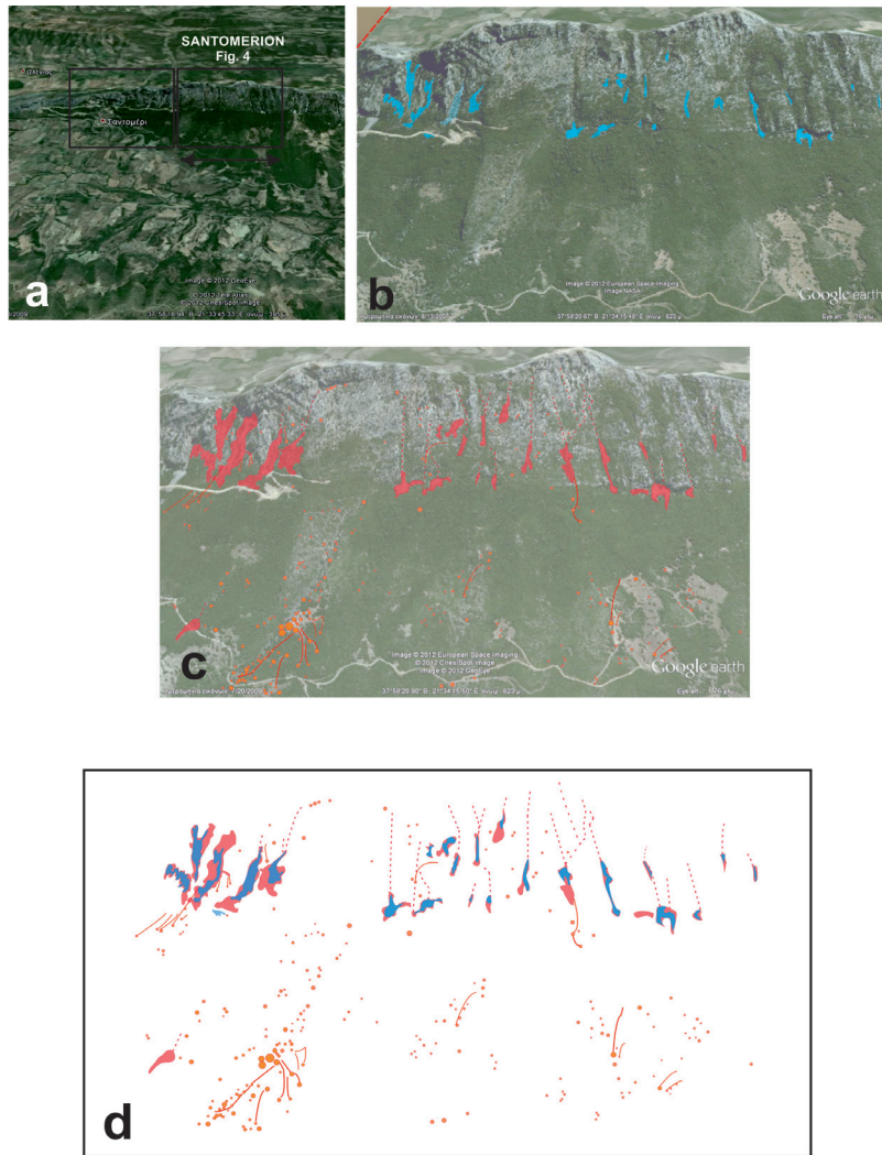
Fig. 4. Temporal evolution of the landslides to the south of Santomerion village for the period 2007-2009. (a) Aerialphoto showing the analyzed area south of Santomerion village in figure 4, aerialphoto was extracted from © Google Earth. (b) Distribution of rock falls, before the earthquake, indicated by the blue areas; the bold red dashed line defines the area where the aerialphoto has low resolution. (c) Distribution of rock falls after the earthquake; red areas correspond to rock fall accumulation zones, the orange dots correspond to isolated blocks and the red lines to their trajectories. (d) Overlapping of pre-earthquake and post-earthquake rock falls around the Santomerion village.
