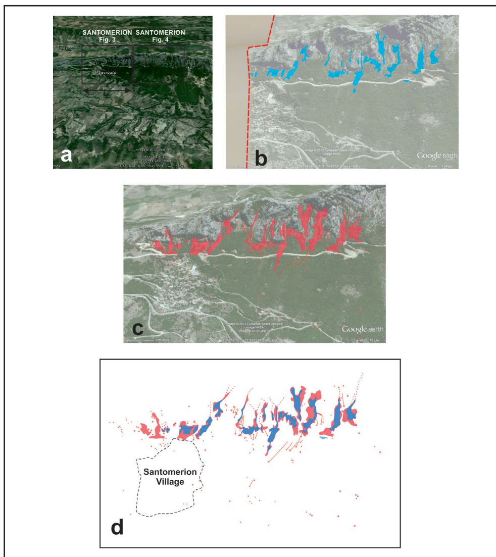
Fig. 3. Temporal evolution of the landslides of Santomerion village for the period 2007-2009. (a) Aerialphoto showing the analyzed area around Santomerion village in figure 3, aerialphoto was extracted from © Google Earth. (b) Distribution of rock falls, before the earthquake, indicated by the blue areas; the bold red dashed line defines the area where the aerialphoto has low resolution. (c) Distribution of rock falls after the earthquake; red areas correspond to rock fall accumulation zones, the orange dots correspond to isolated blocks and the red lines to their trajectories. (d) Overlapping of pre-earthquake and post-earthquake rock falls around the Santomerion village.
