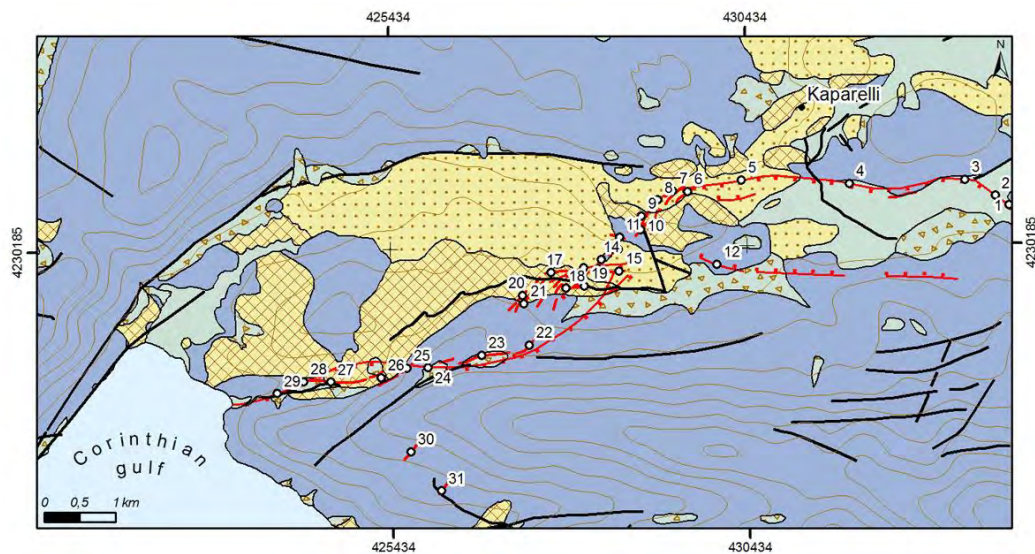
Figure 5 - Geological map of Kaparelli region (northern part of the eastern Corinthian gulf) illustrating the 1981 seismic ruptures (based on the geological map of Greece in scale 1:50.000; Jackson et al., 1982; Rondoyanni & Koukis, 1989). The numbers correspond to the sites where displacement data were available. The geological formations as noted in Figure 4.
