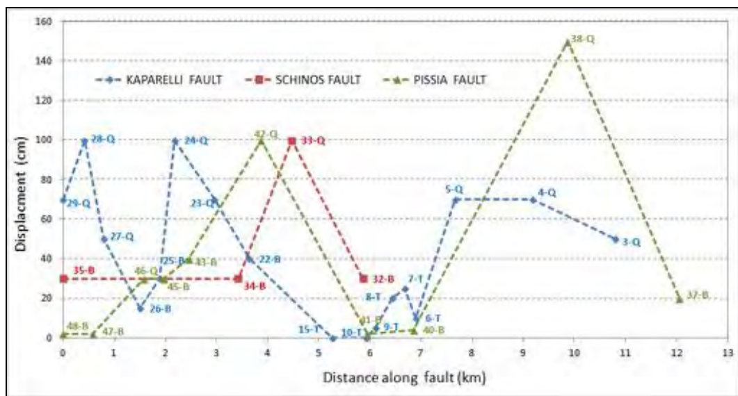
Figure 6 - Coseismic surface displacement along the 1981 reactivated faults (Schinos and Pissia faults are shown in Figure 4; Kaparelli fault in Figure 5). The numbers correspond to the sites noted also in Figures 4 and 5. Sites not presented in Figure 4 correspond to open seismic cracks with no vertical displacement. Lithology notation: B: Bedrock, Q: Quaternary unconsolidated geological formations, T: Transfer zone of Kaparelli fault.
