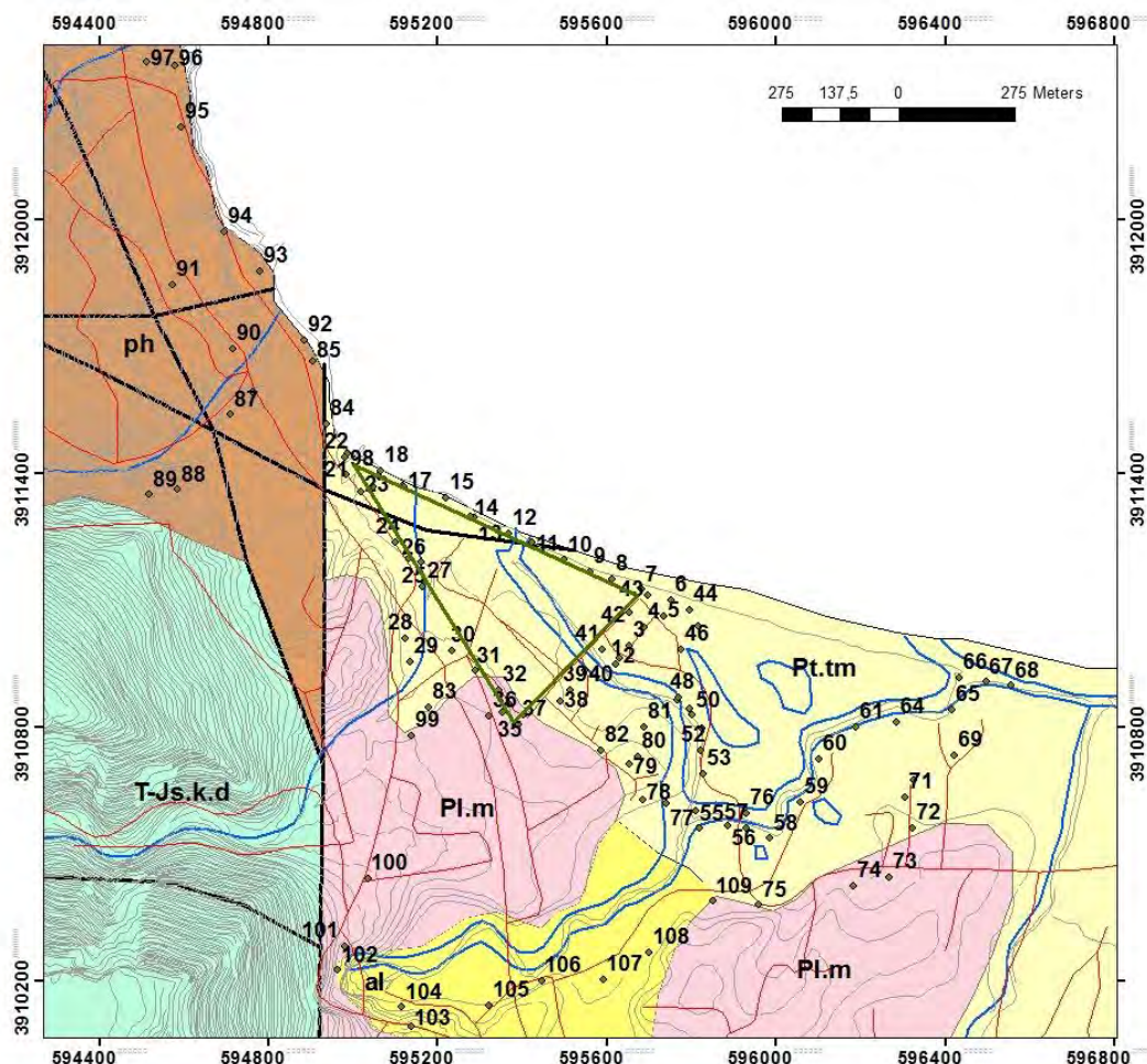
Figure 2 - Geological map of the wider area (according to geological map of IGME). Sympols: al-alluvial sed., Pt.tm-marls, sands and conglomerate, Pl.m- Finikia formation, Ts- Js.Kd - Triassic –Upper Jurassic limestones, dolomitic limestones and dolomites., ph- phyllites, Black line-fault, blue line-drainage net, Green line -power plant, Red line - traffic net, Black circle-sample location.
