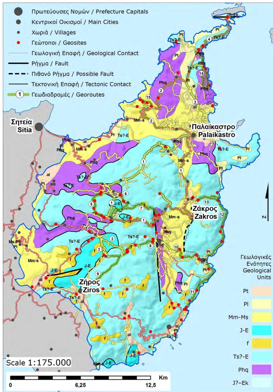
Figure 1 – Simplified geological map of Sitia Nature Park based on Creutzburg et al., 1977 and field studies. Pt, Pleistocene seds.; Pl, Pliocene seds.; Mm-Ms, late Miocene seds.; J-E, Magassa Unit; f, Tripolitsa flysch; Ts?-E, Tripolitsa limestone; Phq, Phyllites-quartzite nappe; J?-Ek, Plattenkalk rocks.
