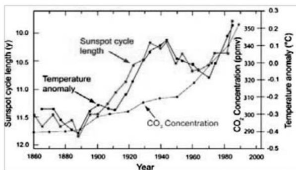
Fig. 20: Correlation between sunspot cycle length, temperature anomalies and atmospheric CO 2 concentration (Friss-Christensen and Lassen, 1991).
