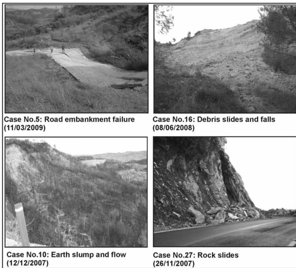
Fig. 3: Landslides identified in the Ilia Prefecture (1950-2005) & (2008).
