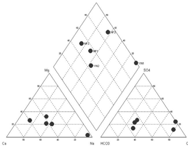
Fig. 3: Piper diagram.
