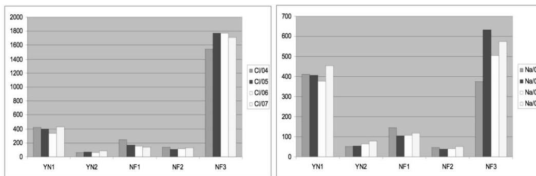
Fig. 5 (left): Cl histogram; (right): Na histogram.
