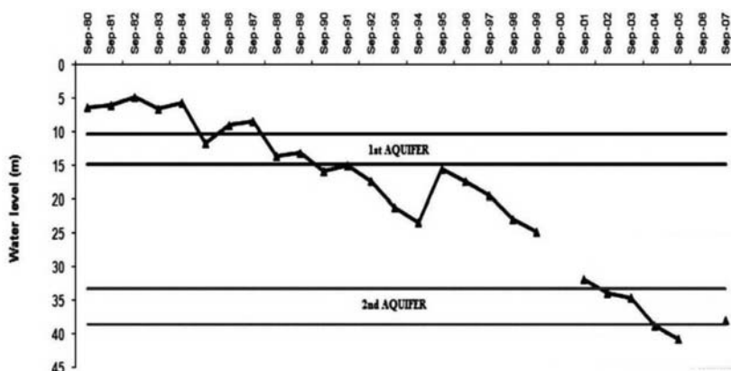
Fig. 6: Ground water table fluctuations with time in Farsala site (Pz46 borehole). The exhaustion of the first two aquifers is obvious.
