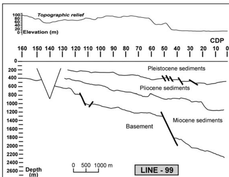
Fig. 4: Interpreted profile of seismic Line-99 (first interpretation).
