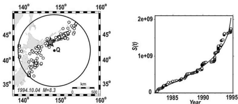
Fig. 1. The circular critical region where accelerating preshocks (open circles) occurred before the generation of the big ( M=8.3 ) mainshock of October 4, 1994 in northern Japan ( 43.7^\circ\text{N} , 147.4^\circ\text{E} ). The star denotes the mainshock epicenter while Q is the center of the circular region (solid circle). On the right of the map, the time variation of the cumulative Benioff strain, S(t) , for the accelerating preshocks is given. The solid line represents fitting to the data of a power-law (relation 1).
