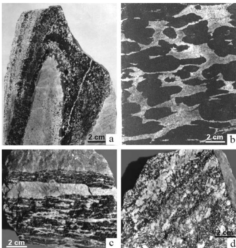
Fig. 3: a: The plastic sindeformed chromitite. The foliation plan of isoclinal fold is parallel to axial plan of folding; b: Nodular chromitite, intensively deformed. The nodules are extended and crushed by strong attraction; Fig. c: The budded chromitite transformed into banded – like shape. The pull-apart lineation is expressed clearly; d: The chromitite intensively deformed, transformed into lenticular – brecciated up to antinodular – shape.
