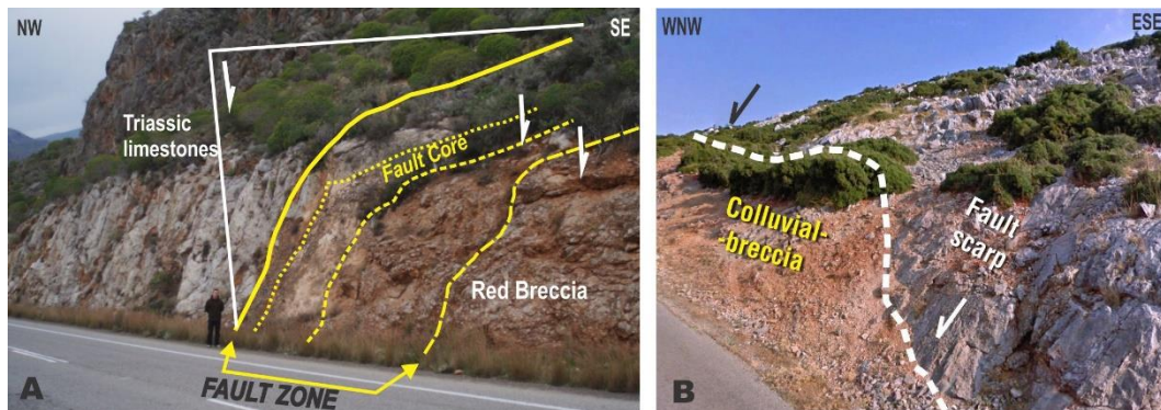
Figure 5 - A) Fault zone detail of the Galaxidi Fault. B) Fault scarp of Kokkinovrachos Fault. Site of images is shown in Figure 3.
