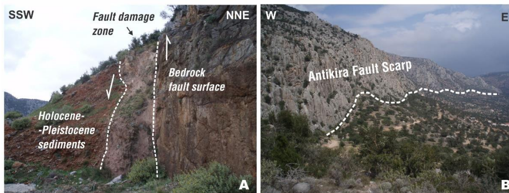
Figure 8 - Examples of normal faulting in the northern Gulf of Corinth Rift. A) Excavation outcrop of Amfissa Fault to the north-west of the city of Amfissa. B) The Antikira Fault scarp in the western side of Antikira Gulf.
