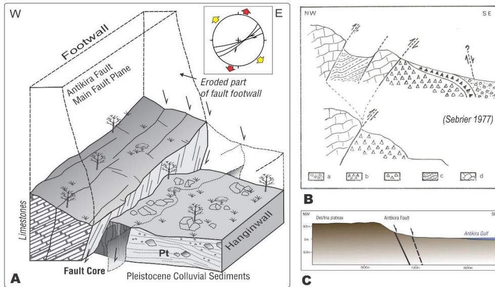
Figure 7 - A) Scetch based on field observations, explaining the mis-labeling of Antikira fault as reverse by Sebrier (1977). The curvature of the fault surface. B) Original sections at Antikira fault from Sebrier (1977). C) Profile of central section of Antikira Fault.
