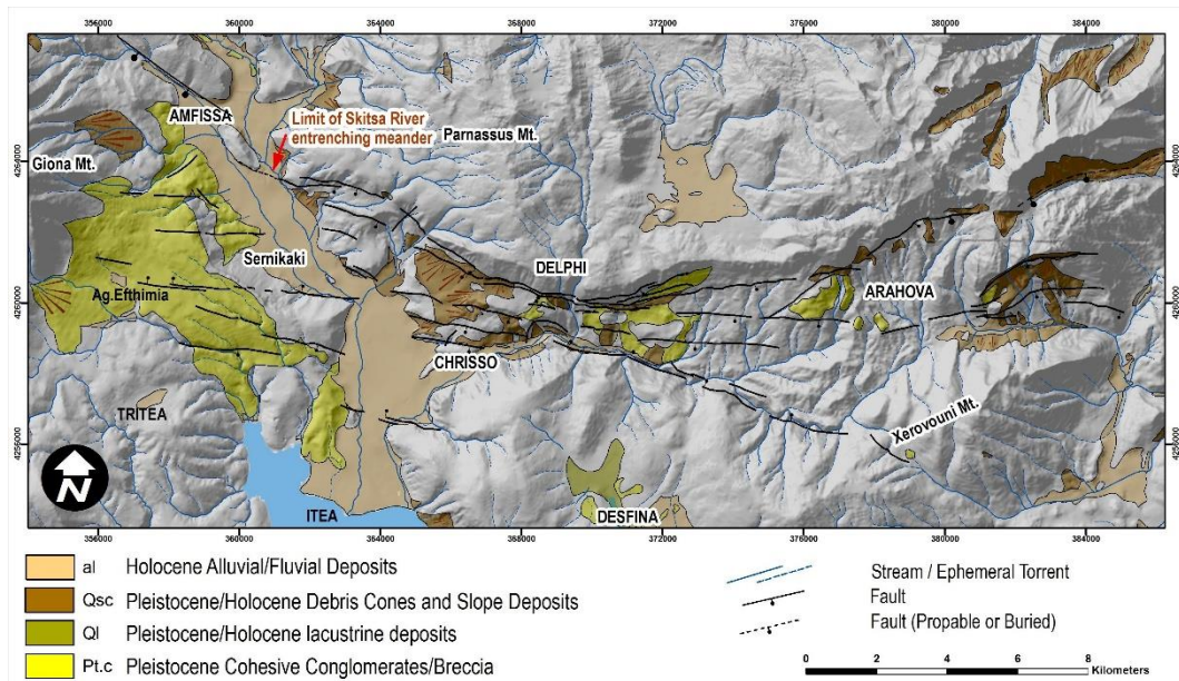
Figure 2 - The Delphi - Arachova Fault zone. Neogene and Quaternary sediments from this study and IGME Geological Maps.
