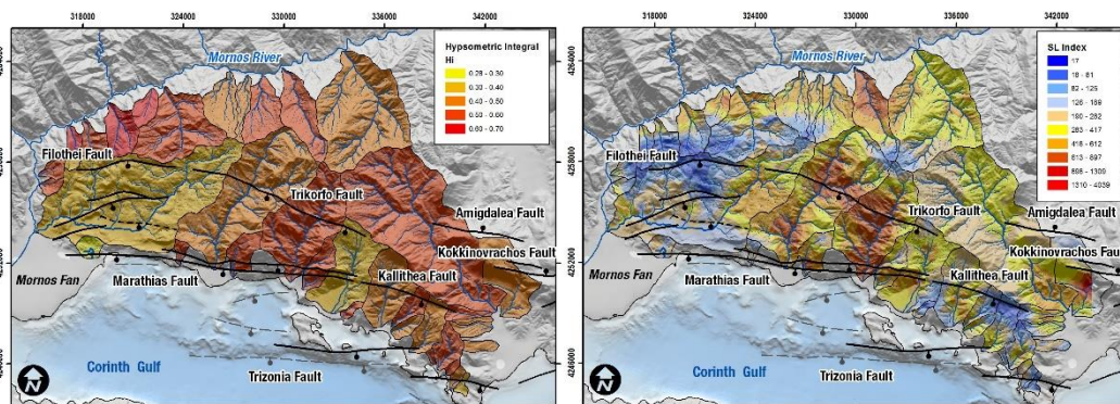
Figure 6 - A) Drainage basins in Trikorfo area, classified with hypsometric integral (Hi) values. Major faults are also shown. B) SL-index values in the same area. High values (red) indicate rapid uplift and erosion in the footwall drainage.
