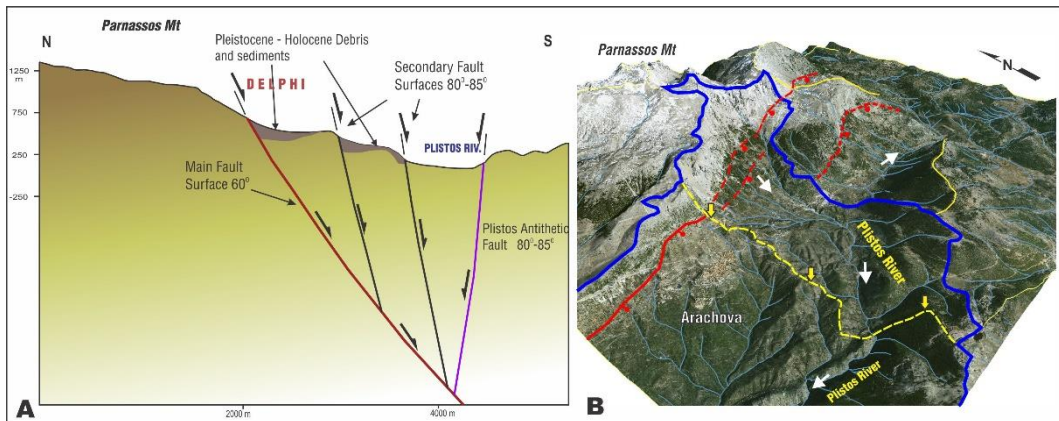
Figure 3 - A) Interpretive section with the tectonic model of the Delphi-Arachova Fault Zone. B) The eastern half of Plistos valley. Plistos basin (blue line) is expanding eastwards, capturing drainage that previously flowed to the east (yellow dotted line). Arachova fault and possible extensions with red line.
