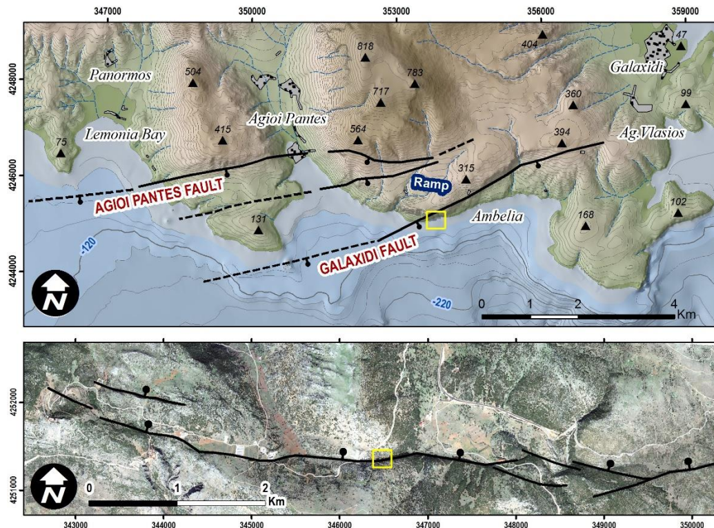
Figure 4 - Above: The Agioi Pantes and Galaxidi Fault Zone. A ramp structure is formed in the overlap area between the two faults. Elevation and bathymetry contour interval is 20m. Below: Kokkinovrachos Fault. Normal Fault scarps mapped with thick black lines and dot on downthrown side.
