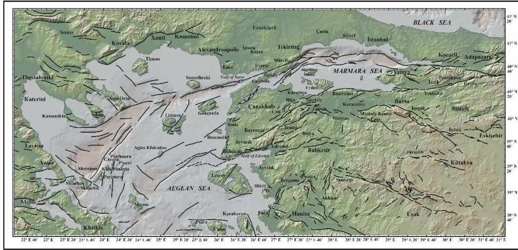
Figure 1 - Active faults in the western Turkey, northern Aegean Sea and northern Greece (active faults were compiled from the following references; in mainland Turkey: Emre et al. (2013) and the references included therein; Troy area: Kürçer et al. (2012); South-west Marmara Sea: Yaltırak (2002); Çanakkale Strait: Gökaşan et al. (2008); active faults at the western part of Gulf of Edremit and its vicinity: Yaltırak et al. (2012); North-eastern Greece: Pavlides et al. (2007); Agios Efstratios fault: Chatzipetros et al. (2012); active faults near Bozcaada: Kürçer et al. (2015).
