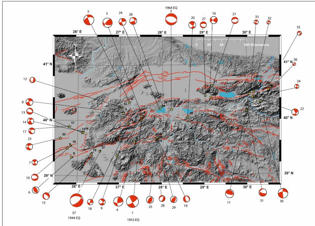
Figure 2 - Focal mechanisms and MT solutions compiled and obtained respectively in the study for the region. The numbers in the map and near the mechanisms indicate earthquake numbers in Table 1 which also contain source parameters.
