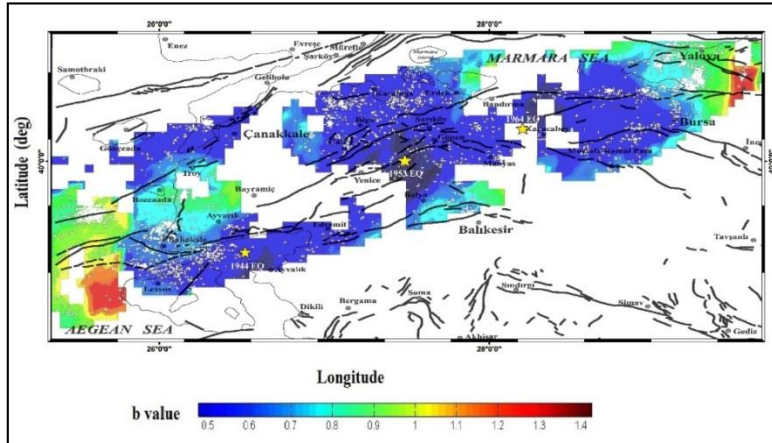
Figure 4 - Map view of spatial distribution of b values using the best combination maximum likelihood method for the time period between 1905-2015 instrumental catalog. The number of earthquakes per sample is 50, the nodal separation is 0.025^\circ , and the radius of the cylindrical sample volumes is R \geq 20 km.
