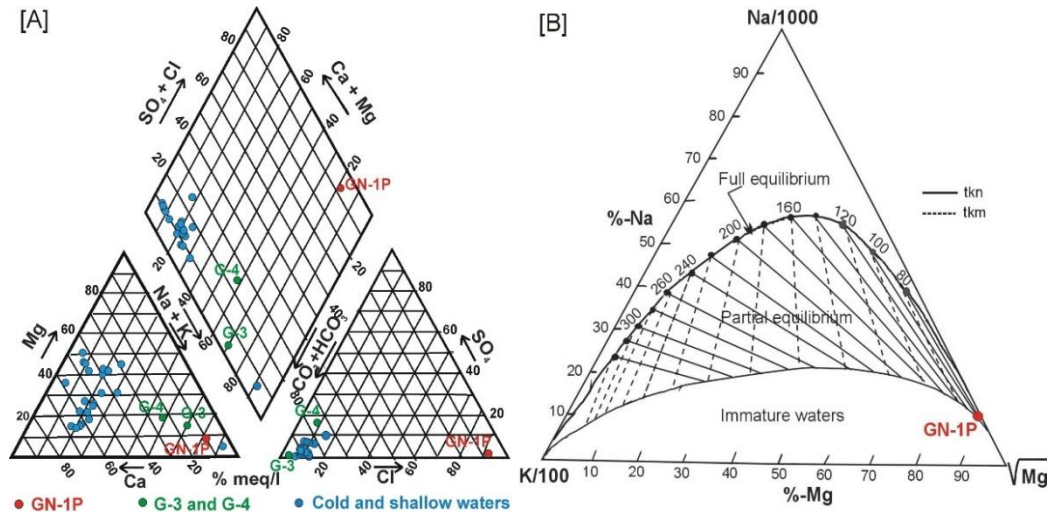
Figure 2 - (A) Piper (1944) trilinear diagram of hot (GN-1P, G-3, G-4) and cold waters from the Alexandria area. (B) Water sample GN-1P is plotted on the Giggenbach (1988) ternary diagram.
