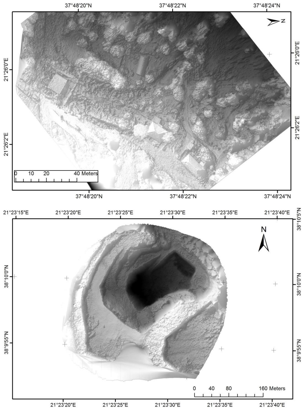
Figure 6 – The DSMs created by the UAV campaigns. The top picture depicts the Analisis landslide DSM and the bottom picture depicts the Araxos open-pit mine DSM.
