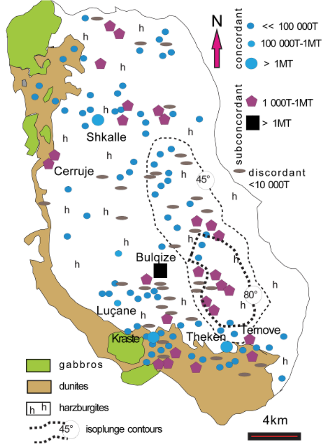
Figure 3 - Distribution of chromite ore bodies and their structural types of Bulqize massif.
