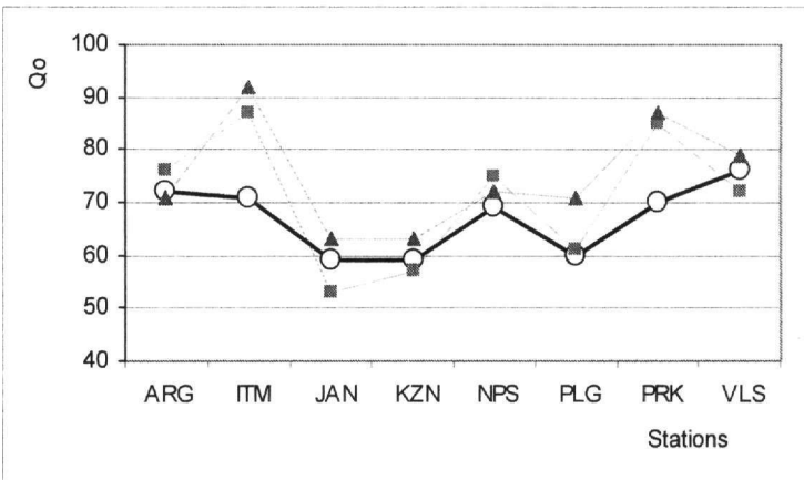
Figure 2. Q_0 at the NOA seismic stations for different ellipsoid semi axis values ( a_2 = 100 \text{ km} , open circles). Full rectangles and triangles represents the Q_0 values for a_2 equal to 130 and 160 km respectively.
