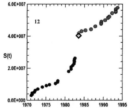
Figure 4. The critical areas of the earthquakes with code numbers 10, 11, 12 of table 1 (left) and the corresponding time variations of the cumulative Benioff strain, S(t) , released by all M \geq M_{min} shocks which occurred in the critical areas during the examined time periods (right) (Kourouzidis 2003). Explanation as in figure 1.
