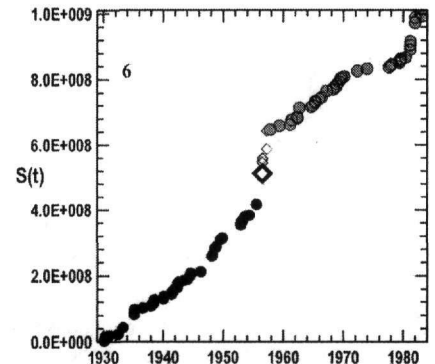
Figure 2. The critical areas of the earthquakes with code numbers 4, 5, 6 of table 1 (left) and the corresponding time variations of the cumulative Benioff strain, S(t) , released by all M \geq M_{\min} shocks which occurred in the critical areas during the examined time periods (right) (Kourouzis 2003). Explanation as in figure 1.
