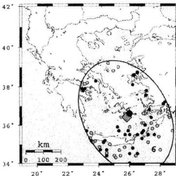
Figure 2. The critical areas of the earthquakes with code numbers 4, 5, 6 of table 1 (left) and the corresponding time variations of the cumulative Benioff strain, S(t) , released by all M \geq M_{\min} shocks which occurred in the critical areas during the examined time periods (right) (Kourouzis 2003). Explanation as in figure 1.
