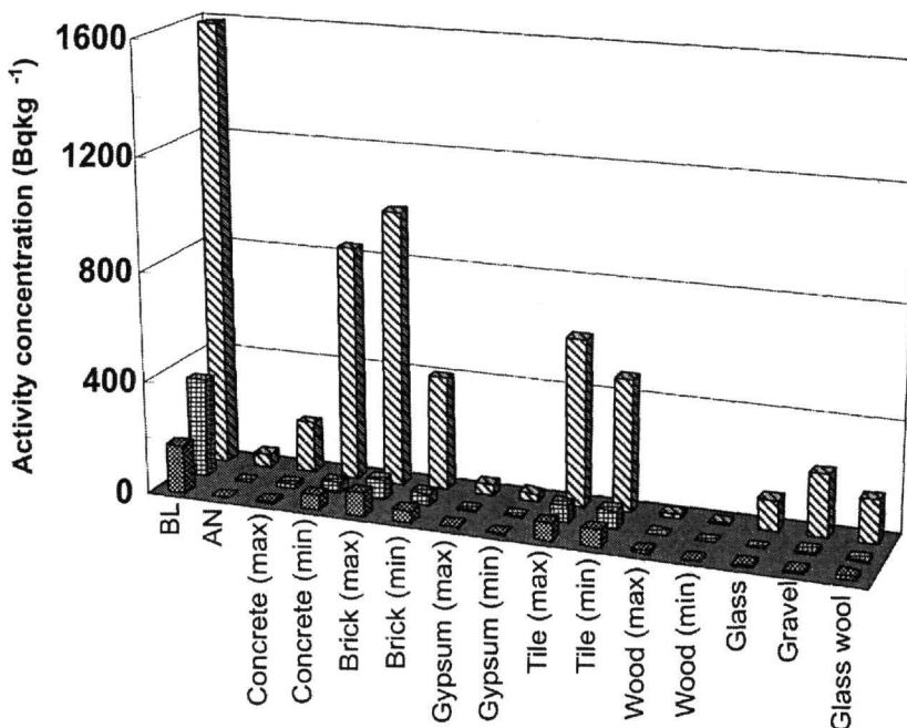
Figure 2. The activity concentrations of ^{226}\text{Ra} , ^{232}\text{Th} and ^{40}\text{K} ( \text{Bq kg}^{-1} ) of the granite samples BL (Balmoral) and AN (Africa nero), having the maximum and the minimum annual effective dose D_a among the examined samples, are compared to maximum (max) and minimum (min) activity concentrations of different building materials (Zikovsky & Kennedy 1992). Symbols as in figure 1.
