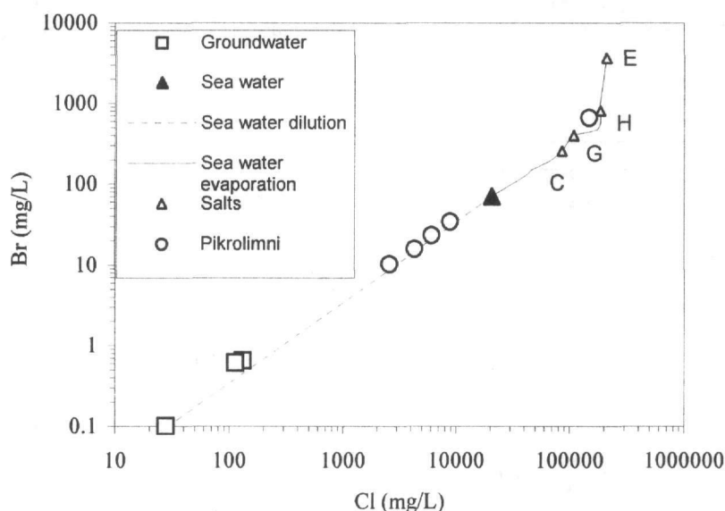
Fig. 2: \text{Cl} versus \text{Br}^- contents of the water (groundwater and brine) of Pikrolimni area. Open triangle the domain of the salts (C: calcite, G: gypsum, H: halite, E: epsomite).
