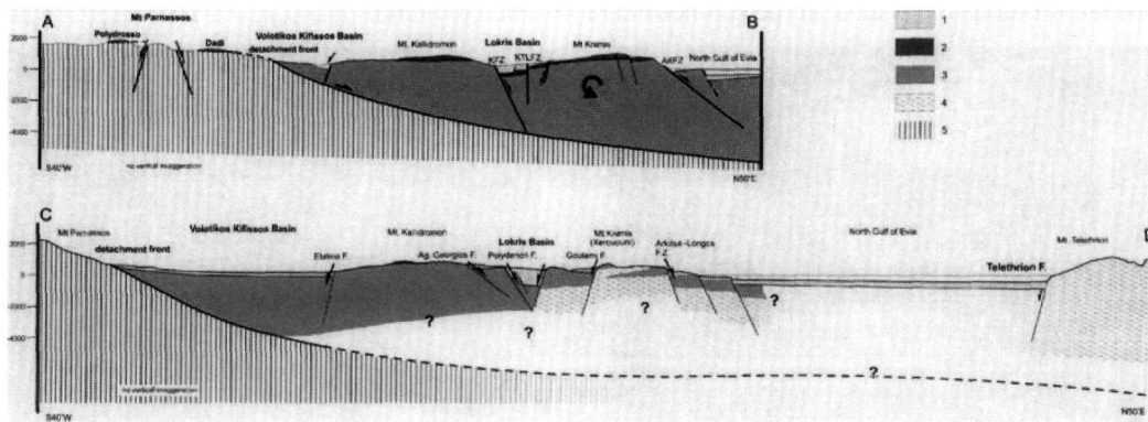
Figure 7 - Interpretative cross-sections through the Lokris and Voiotikos Kifissos Basins (see Fig. 1 for location). 1: Synrift deposits (Pliocene- Quaternary); 2: Ophiolite suite; 3: Sub-Pelagonian Unit; 4: volcaniclastic complex and basement of the SPU; 5: “Lower Plate” formations, which correspond (at least in the western parts) the Parnassos Unit. The formation of both VKB and LB is attributed to the NE-ward sliding on the PDF. Section AB demonstrates the block rotation of Mt Knimis, resulting in the low dips of the AKFZ and the northerly dips of the originally S-dipping KTLFZ. This pattern is confirmed by the systematic southward lowering of the base of the ophiolite nappe. Section CD shows the uplifted volcaniclastic basal complex of the SPU, at the area of Melidoni, which may be linked to the SPU basement, outcropping just across the N. Gulf of Evia, on Mt Telethron. The suggested shallowing of the detachment surface beneath the Gulf is believed to reflect the crustal thinning observed at this area (Makris et al. 2001)
