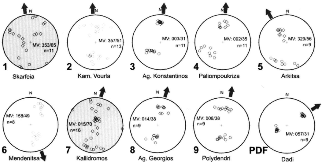
Figure 4 - Lower hemisphere stereographic projections of fault-slip data. Diamonds are lineations on fault planes, circles are poles to planes. MV: mean lineation orientation from Fischer statistics. White stereonets are for data from the main fault planes; gray ones for data from footwall fault arrays within ~10 m from the main fault plane. For location of measurement stations see Figures 1 and 2
