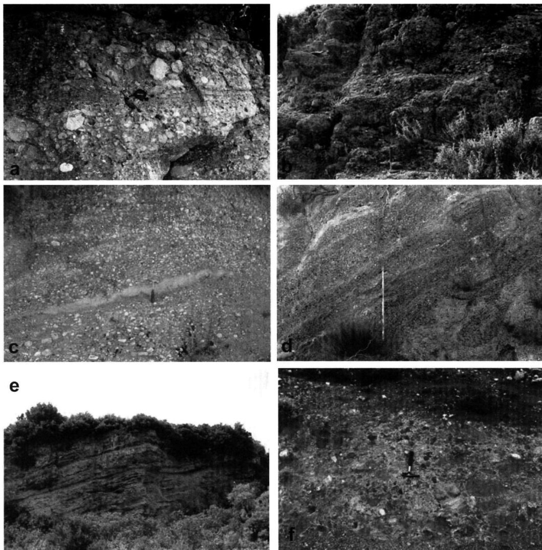
Figure 3 - Field photos from outcrops in Lokris. (a) the basal members and (b) the ologimictic conglomerates of the Karya fm. Lens cap and hammer for scale; (c) typical exposure of the Agnandi fm; (d) The steeply dipping fine conglomerates of the Renginon fm. Dip direction is SSW; (e) the compact carbonate breccias that form the upper member of the Mendenitsa formation; (f) typical exposure of the reddish conglomerates in Drymaia
