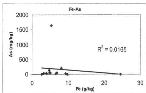
Figure 2. Iron vs. Arsenic in Kavala soils.
