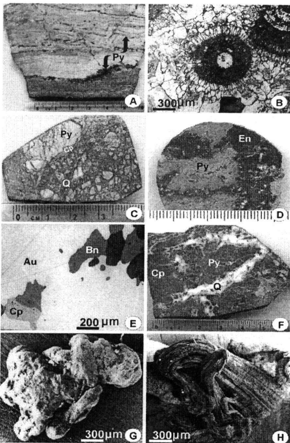
Figure 4. Early and main mineral assemblages: A- dacite tuff from Krassen with pyrite (Py) lamination (scale in cm); B- zonal texture of colloform pyrite (Early pyrite-quartz assemblage) from Elshitsa deposit; C- pyrite (Py) breccia replaced and crosscutted by chalcopyrite (Cp) and quartz (Q) from the chalcopyrite-pyrite assemblage; D- Early pyrite (Py) replaced by enargite (En) from Krassen deposit (scale in cm); E- gold (Au) in assemblage with bornite (Bn) and chalcopyrite (Cp), Radka deposit; F- early pyrite (Py) and (Cp) chalcopyrite chalcopyrite-pyrite assemblage) crosscutted and replaced by the late vein quartz (Q), (scale in cm); G- gold extracted from bornite-chalcopyrite ore, Radka deposit, SEM; H - native silver from Radka deposit, SEM.
