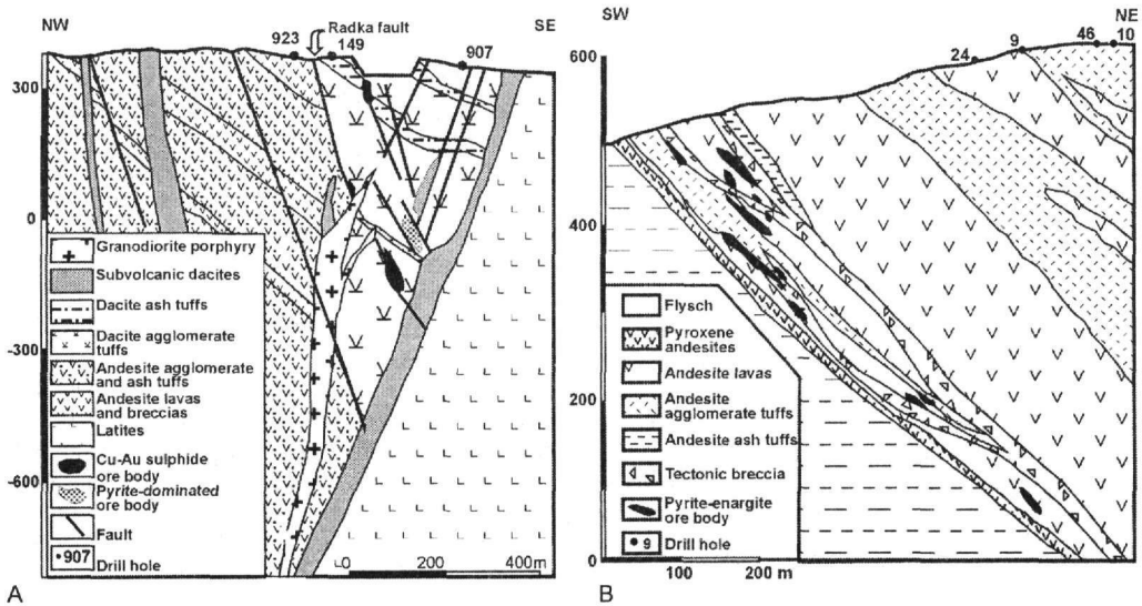
Figure 3. Cross-sections of Radka (A) and Krassen (B) Cu-Au epithermal deposits.
