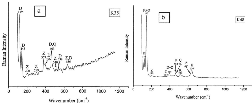
Figure 6. FT-Raman spectrum of the 100-1200 \text{cm}^{-1} region of highly altered rhyolitic rock from Kefalos (a) and Asfendiou (b). Z=Zunyite, D=dickite, K=kaolinite, Q=quartz.
