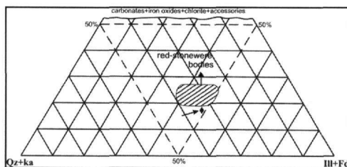
Figure 12 - Ternary diagram for ceramic bodies: “Quartz+kaolinite/chlorite+carbonates+iron oxides/illite-muscovite+feldspars”
