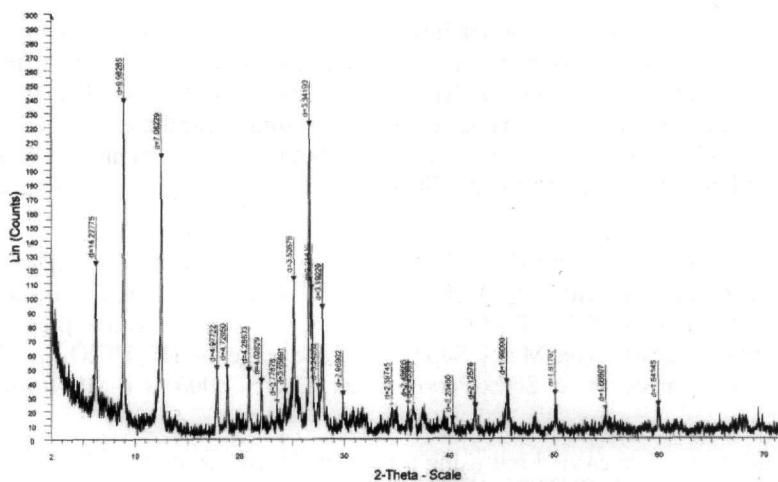
Figure 3 - X ray diffraction diagram of A9a sample
