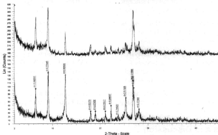
Figure 4 - X ray diffraction diagrams of A9a sample, before an after heating up to 550 °C
