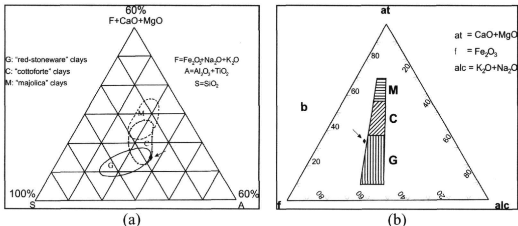
Figure 11 - (a) Ternary diagram \text{SiO}_2/\text{Al}_2\text{O}_3+\text{TiO}_2/\text{Fe}_2\text{O}_3+\text{MgO}+\text{CaO}+\text{K}_2\text{O}+\text{Na}_2\text{O} , (b) Ternary diagram \text{Fe}_2\text{O}_3/\text{MgO}+\text{CaO}/\text{K}_2\text{O}+\text{Na}_2\text{O}
