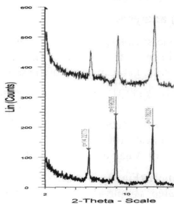
Figure 5 - X-ray diffraction diagram of sample A9a after its saturation with glycol
