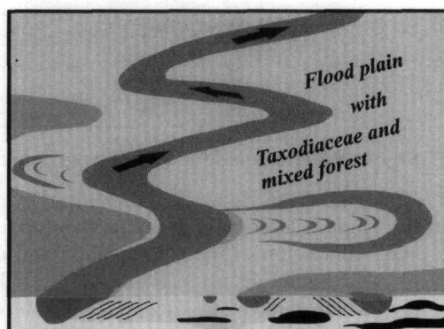
Figure 10 - Paleocological reconstruction of the general area
