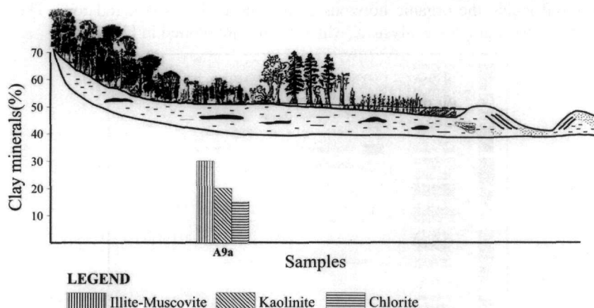
Figure 9 - Distribution of clay minerals in the paleoenvironment of the studied area
