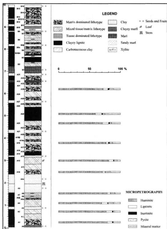
Figure 8 - Micro- and macropetrographical analysis of coal seams in studied area
