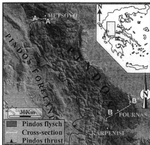
Figure 1. Simplified geological map showing the studied cross-sections.
