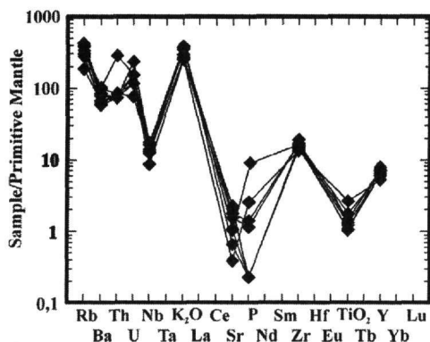
Figure 10. Trace element \epsilon abundance normalised to primitive mantle. (a) Phengite-orthogneisses are characterized by strong negative Nb, \text{TiO}_2 and P anomalies. (b) Amphibole-epidote-albite-orthogneisses are characterized by moderate negative Nb, \text{TiO}_2 and P anomalies. Diamonds: phengite orthogneisses; filled boxes: dioritic orthogneisses; filled circles: granodioritic orthogneisses. The normalizing values are from Sun & McDonough (1989).
