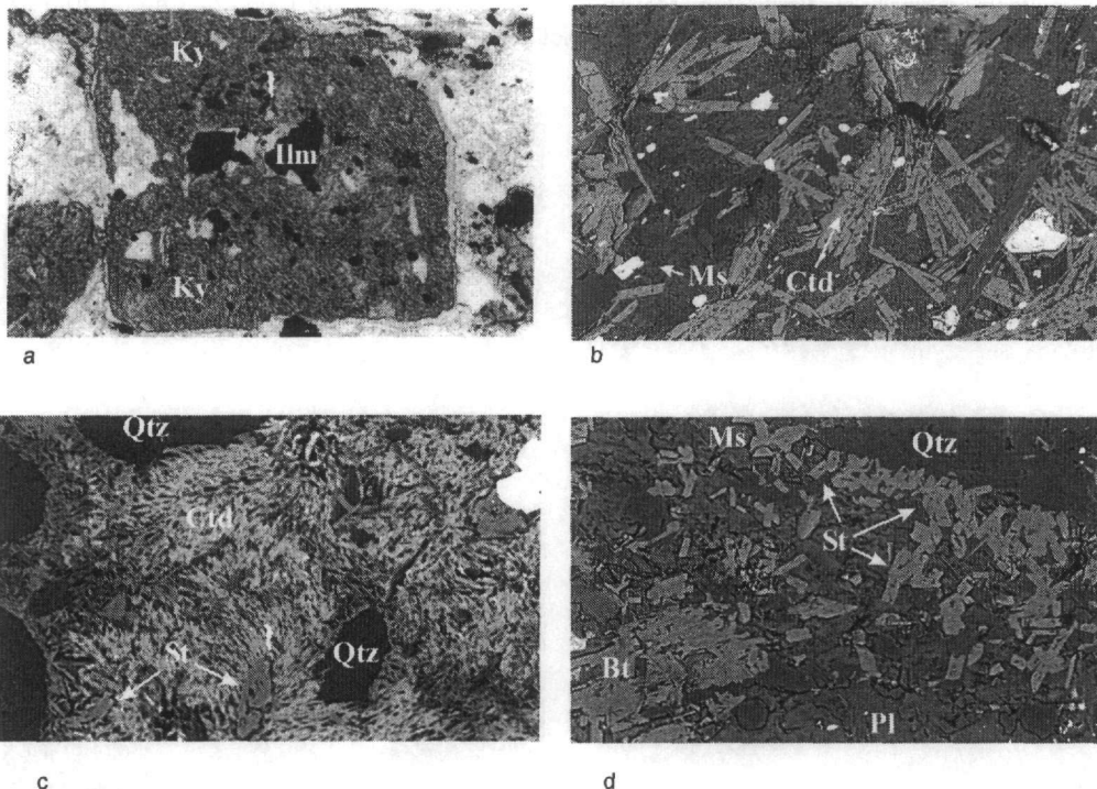
Fig. 4: Andalusite-sillimanite-(cordierite)-gneisses: Alpine overprint.
