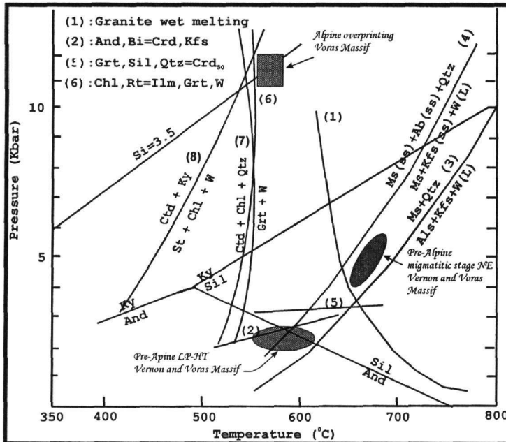
Fig. 5: P-T diagram with reaction curves in a pelitic system, taken from Spear (1995). Isoleth Si=3.5 is from Massonne and Schreyer (1987). Reaction curves 2 and 5 are taken from Mposkos et al., 2001; reaction curves 6, 7 and 8 are calculated with the TWEEQU software (Berman, 1991) using analyzed mineral composition.
