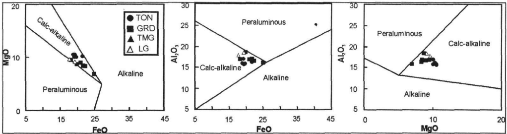
Figure 5. Plot of the biotites from the Brnjica granitoids on the Abdel-Rahman (1994) discrimination diagrams.
