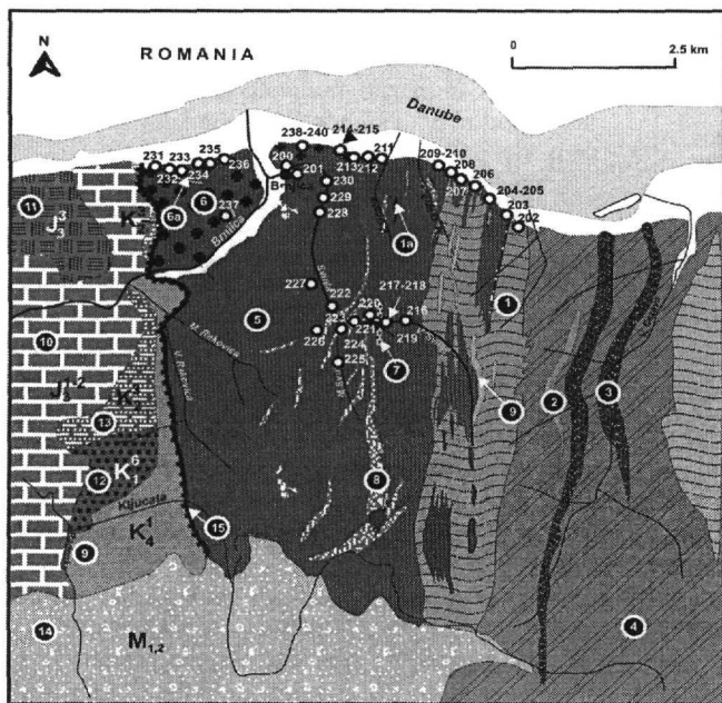
Figure 3. Simplified geological map of the Brnjica granitoids and surrounding area. 1. Gneiss and mica schist (Lower to Middle Proterozoic); 1a. Quartzite 2. Gneiss-granite; 3. Amphibolite (Upper Proterozoic); 4. Greenschist; 5. Tonalite and Granodiorite; 6. Biotite Granodiorite and Granite; 6a. Aplite; 7. Two-mica granite; 8. Contact metamorphosed mica schist and gneiss; 9. Leucogranite, aplite, pegmatite; 10. Limestone; 11. Marly limestone, dolomite and marl; 12. Marly limestone, marl; 13. Conglomerate, sandstone, sometimes glauconitic and claystone; 14. Conglomerate, sandstone and sandy claystone, marl (Neogen-Miocen); 15. Thrust; ● - Location of samples analyzed in this study.
