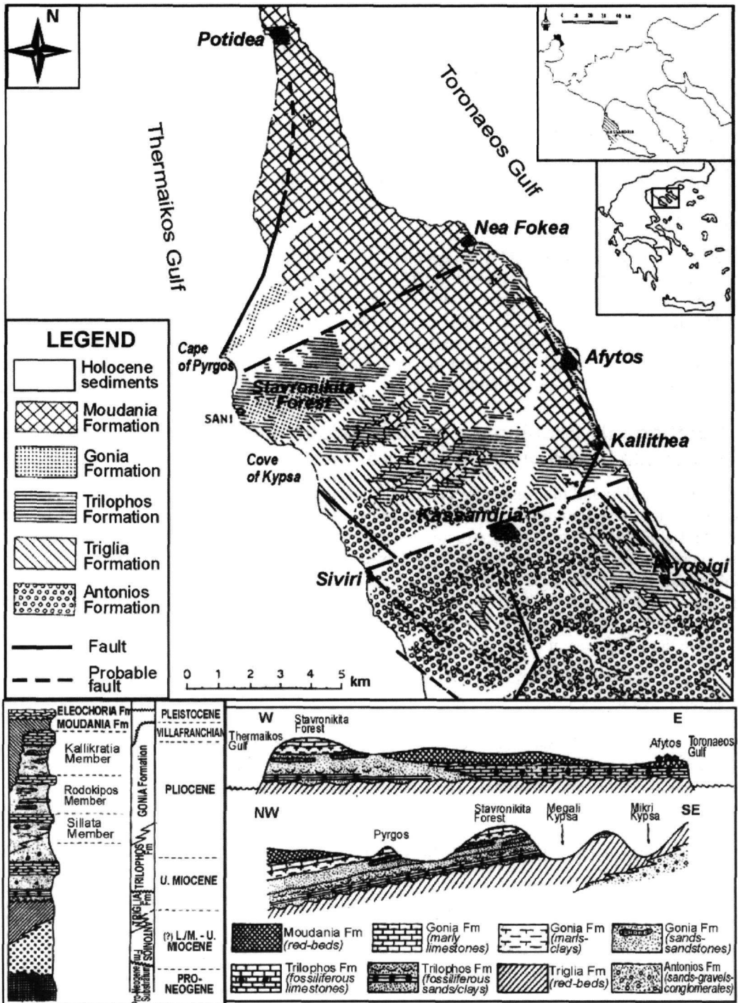
Figure 1 - Above: Geological map of the Sani-Afytos-Kassandra area (Syrides 1990) with the addition of some main and probable faults by Mountrakis et al. (1993). Below: Lithostratigraphic column and two geological cross-sections through the Kassandra Peninsula in the research area (Syrides 1990)
