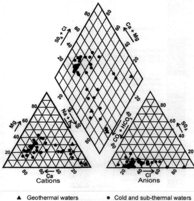
Figure 6 - Presentation of the values of chemical analyses of the waters (cold, sub-thermal and geothermal) from the Afyotos - Sani area on a trilinear diagram according to Piper (1944)
