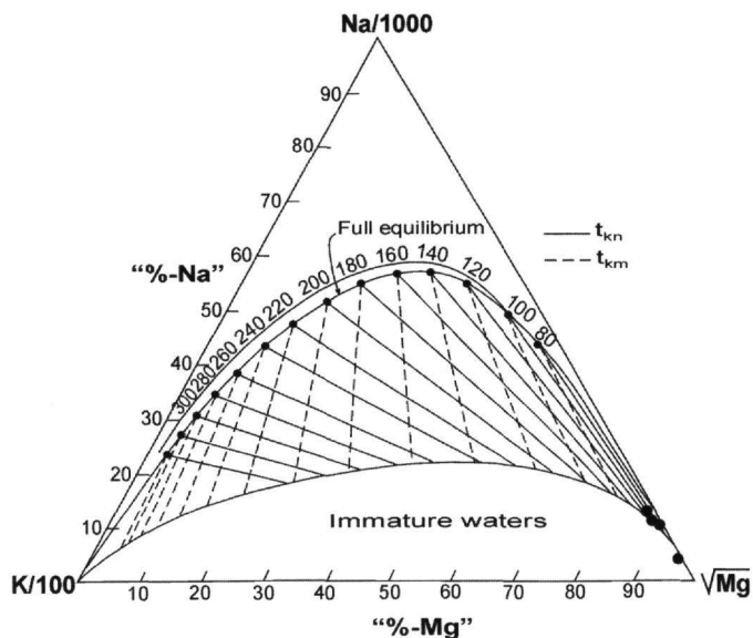
Figure 7 - Evaluation of Na-K-Mg temperature for the geothermal waters KG-2, KG-4, KG-5 and KG-2P on diagram after Giggenbach (1988)
