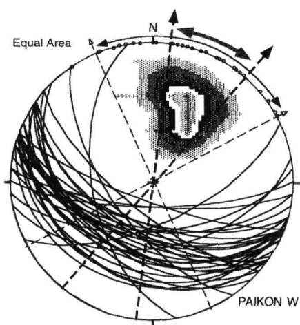
Fig. 4 : Stereographic projection of the bedding planes (So), shear planes (C) and cleavages planes (S1) whose relations show a top-to-the NNE vergence of the western Paikon slices (Equal area, lower hemisphere projection).
