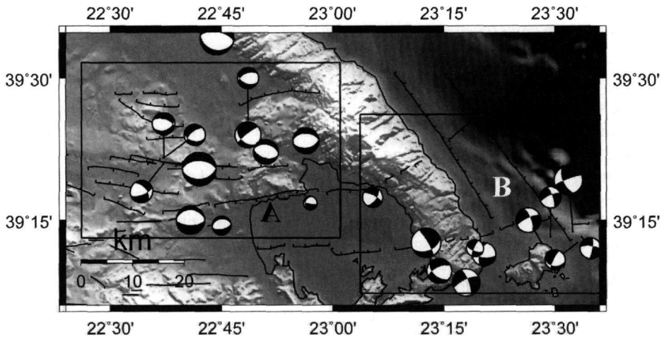
Figure 10 – Locations and focal mechanisms of local earthquakes (Hatzfeld et al. 2001)
