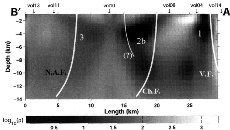
Figure 8 – Goelectric image of the schizosphere along transect A-B', obtained from two-dimensional inversion. Depths refer to m.s.l. The outline numbers indicate conductors correlated between transects A-A' and B-B' (see also Fig. 7)
