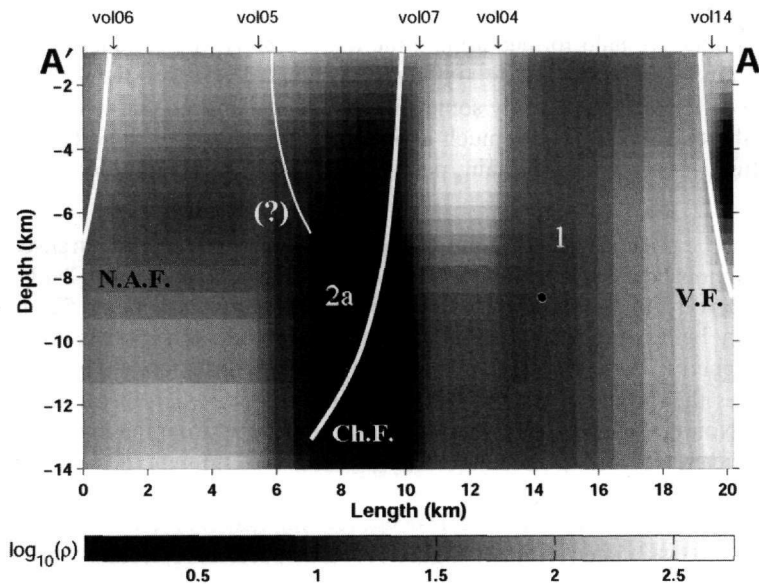
Figure 7 – Goelectric image of the schizosphere along transect A-A', obtained by two-dimensional inversion. Depths refer to mean sea level. The numbers indicate conductors correlated between transect A-A' and A-B' (also see Fig. 7)
