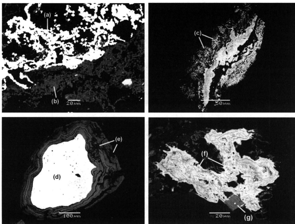
Figure 6 - SEMs in back-scattered mode of selected bright particles: (a) Pb- alunite (corkite), (b) jarosite, (c) pyromorphite, (d) metallurgical slag containing Si, Fe, Pb, (e) pyromorphite, (f) Fe-Mn oxide enriched in heavy metals, (g) oxidised pyrite pseudomorph
