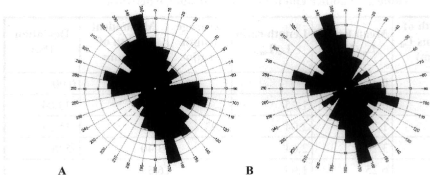
Figure 5 – Rose diagrams of frequency (A) and density (B) for thrusts and overthrusts
