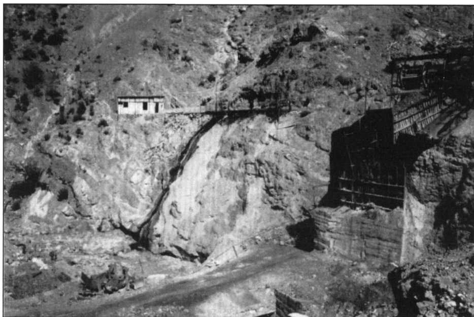
Figure 2 - Acid waters flowing from the Spaci Repsi Mine area
