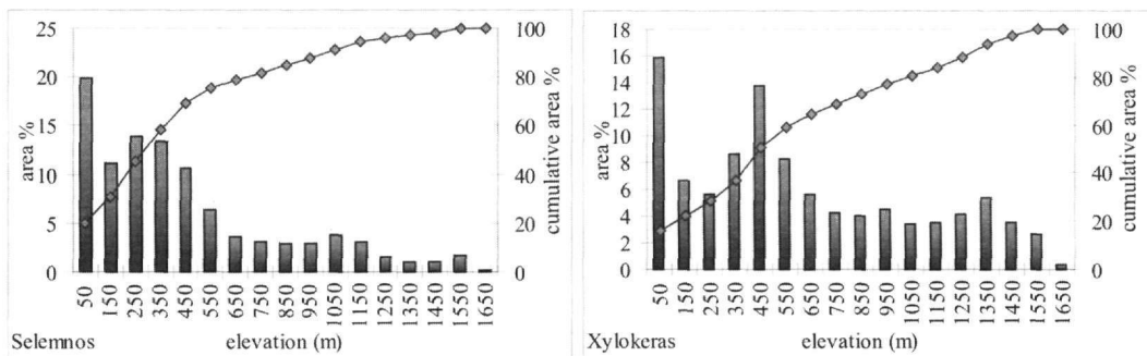
Figure 3 – Area-elevation curves of Selemnos and Xylokeras basins
