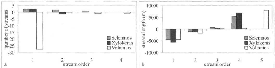
Figure 6 – Diagram showing the deviation of the number (a) and length (b) of streams
