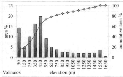
Figure 4 – Area-elevation curve of Volinaios basin
