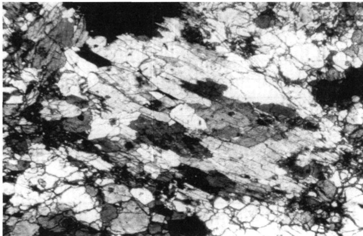
Figure 3 - Microscopic image of granulated harzburgite with tremolite (crossed Nichols)
