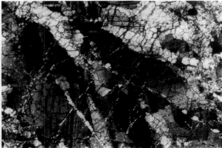
Figure 2 - Microscopic image of tectonized harzburgite taken from the appearances northern of village Papades. Elongated olivine crystals are distinguished presenting undulose extinction (crossed Nichols)
