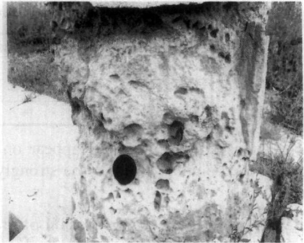
Figure 13 - Severe decay of bottom column piece constructed of type III sandstone and shape alteration
