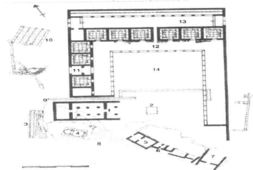
Figure 4 - Plan of Artemis Temple area. 1. Temple, 5. Iphigeneia heroon, 6. Iphigeneia tomb, 7. Sacred house, 12. Stoa 14. Courtyard
