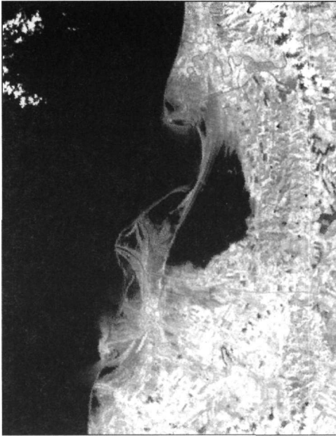
Landsat MSS 1978
