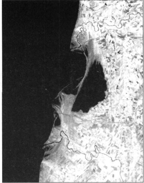
Landsat MSS 1981
