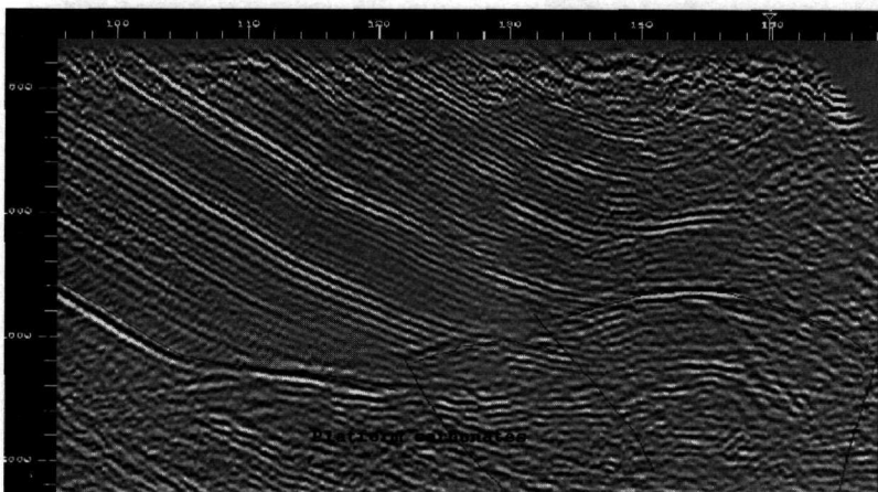
Fig. 5. Seismic line IV-IV, across platform carbonates
